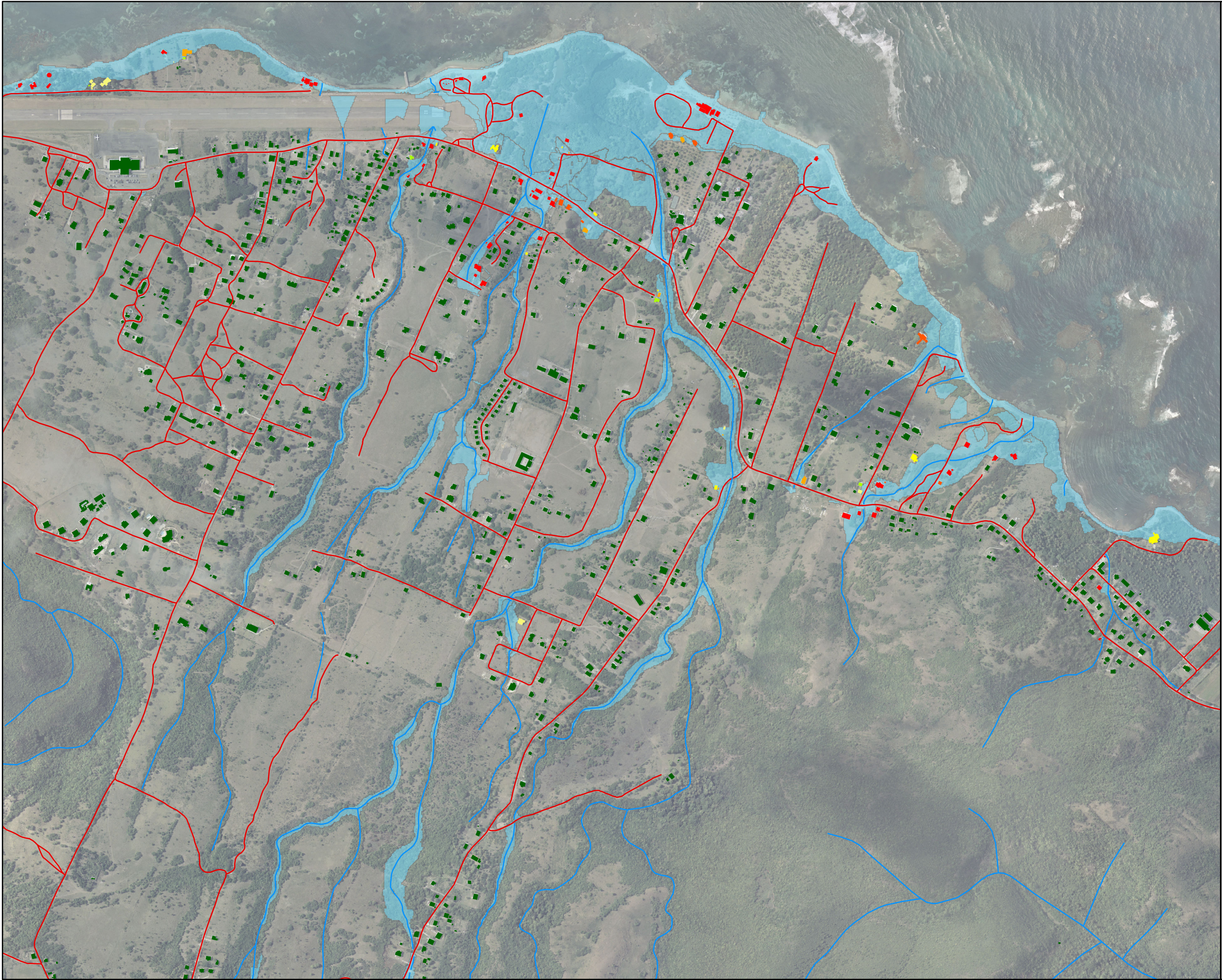
FIGURE N - 6 Buildings Flooded - Scenario A - - Newcastle SLR 0.5m, +10% event rainfall Task 4: Simulation of Pertinent Drainage Scenarios Nevis Drainage Master Plan
